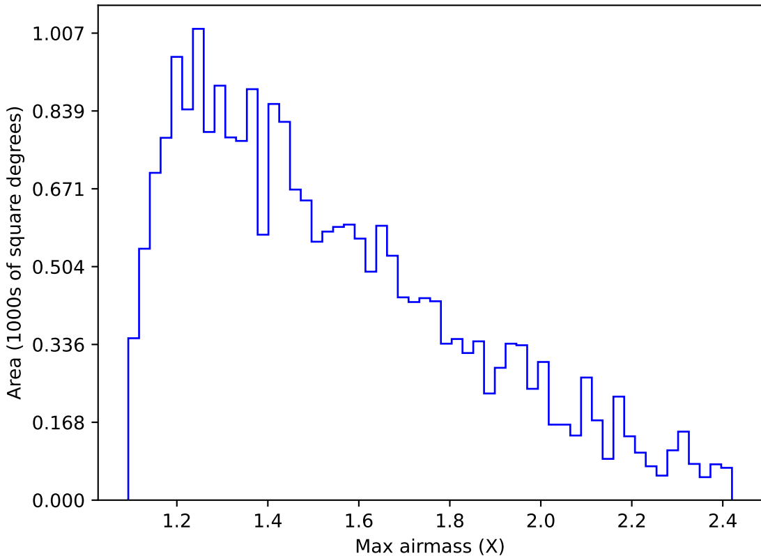
too_elab_heavy_r128_d3_gz_v3.4_10yrs Yr 1 u band: Max airmass
