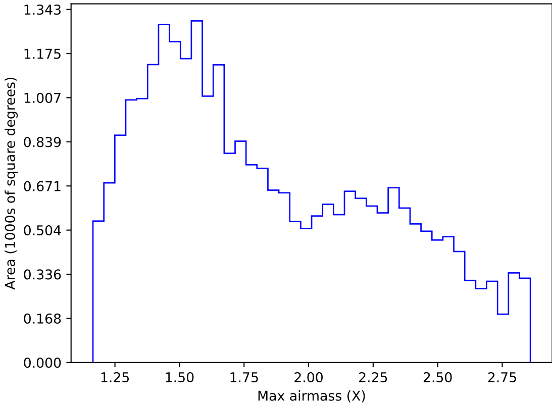
too_elab_heavy_r128_d3_gz_v3.4_10yrs Yr 1 i band: Max airmass
