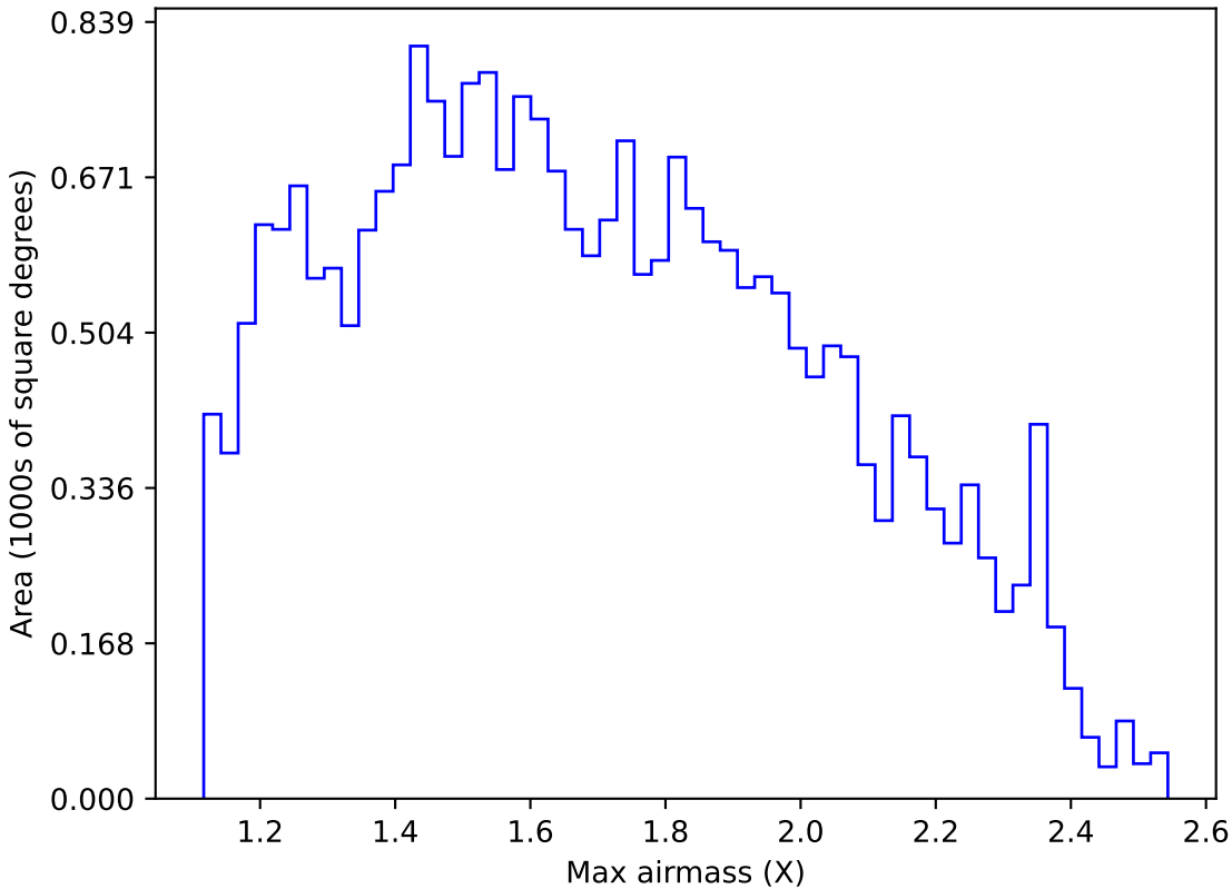
too_elab_heavy_r128_d3_gz_v3.4_10yrs Yr 1 g band: Max airmass
