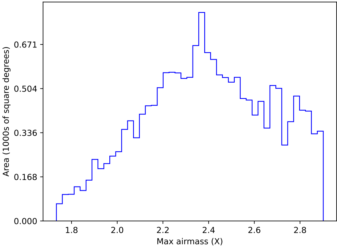
too_elab_heavy_r128_d3_gz_v3.4_10yrs WFD z band: Max airmass
