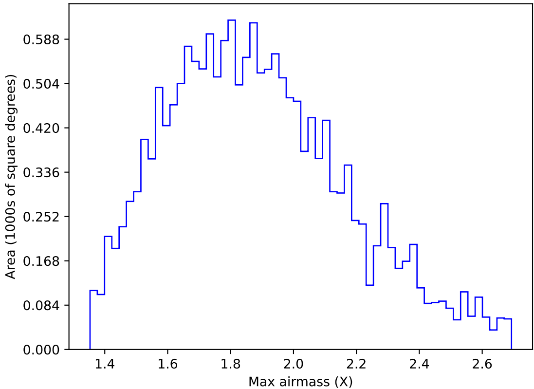
too_elab_heavy_r128_d3_gz_v3.4_10yrs WFD u band: Max airmass
