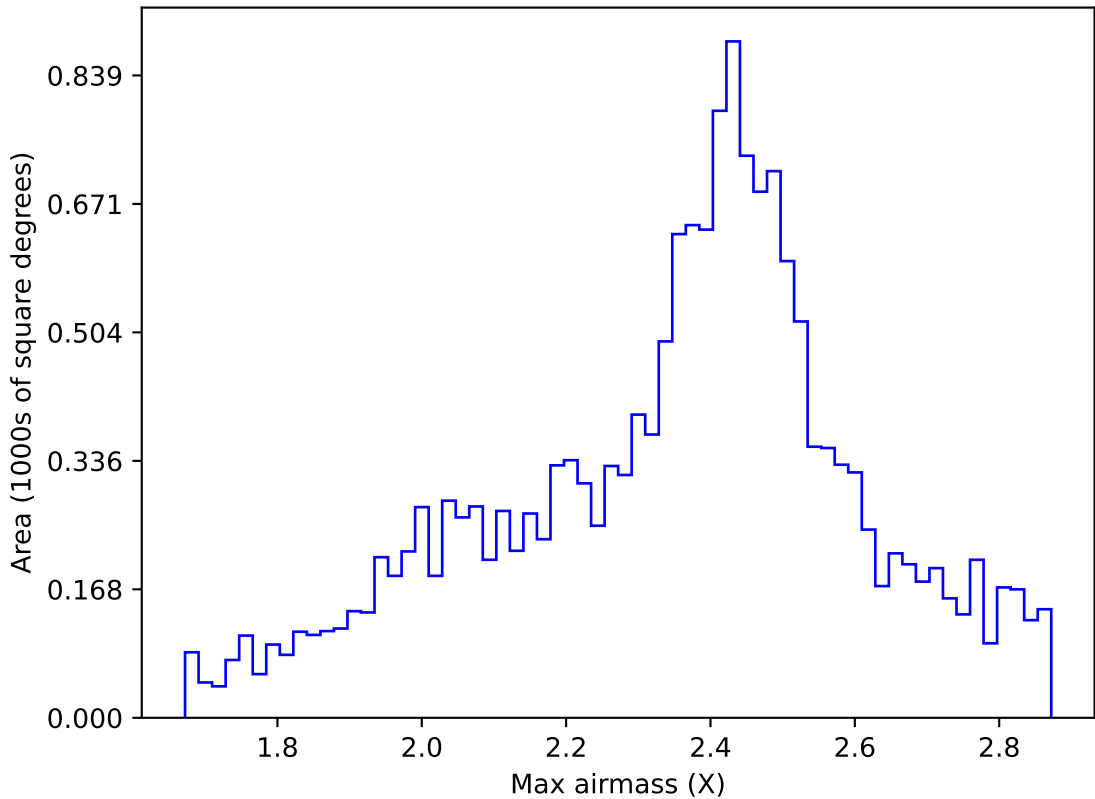
too_elab_heavy_r128_d3_gz_v3.4_10yrs WFD r band: Max airmass
