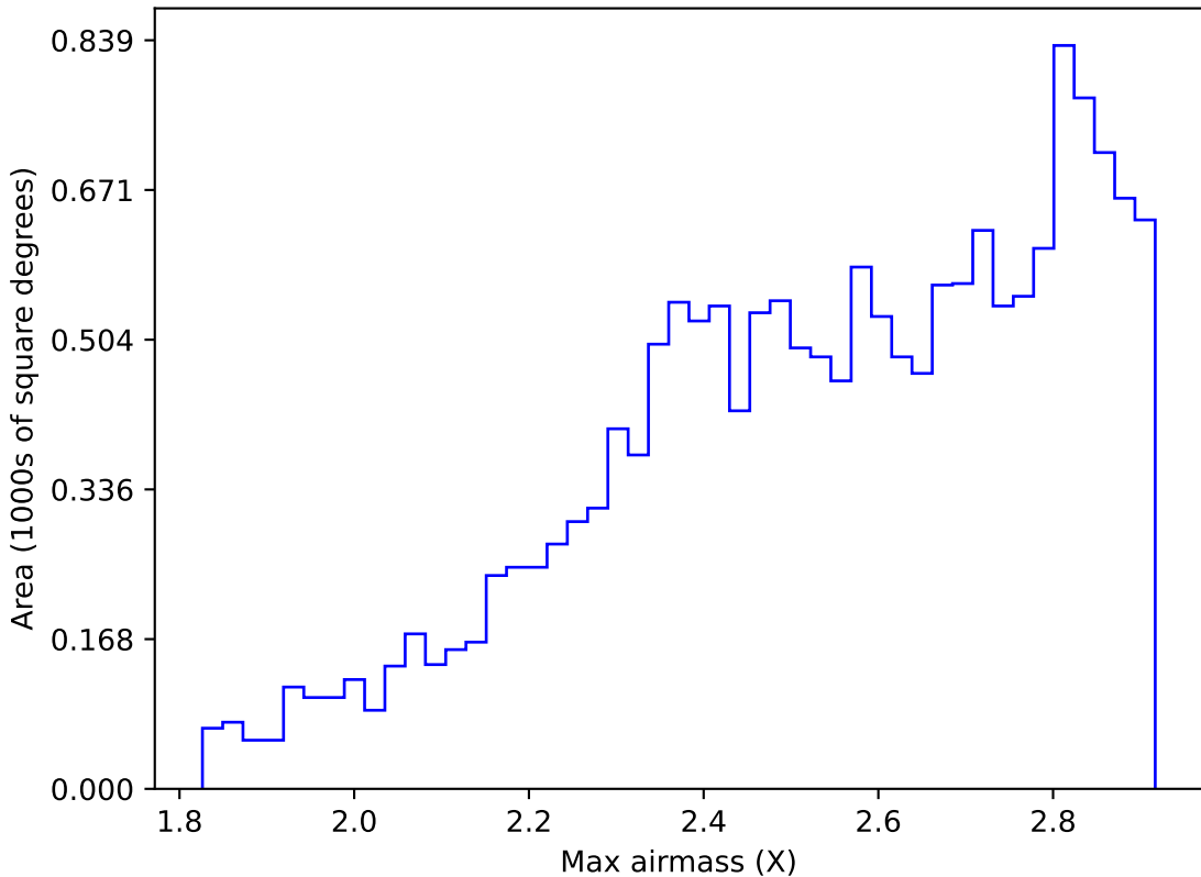
too_elab_heavy_r128_d3_gz_v3.4_10yrs WFD i band: Max airmass
