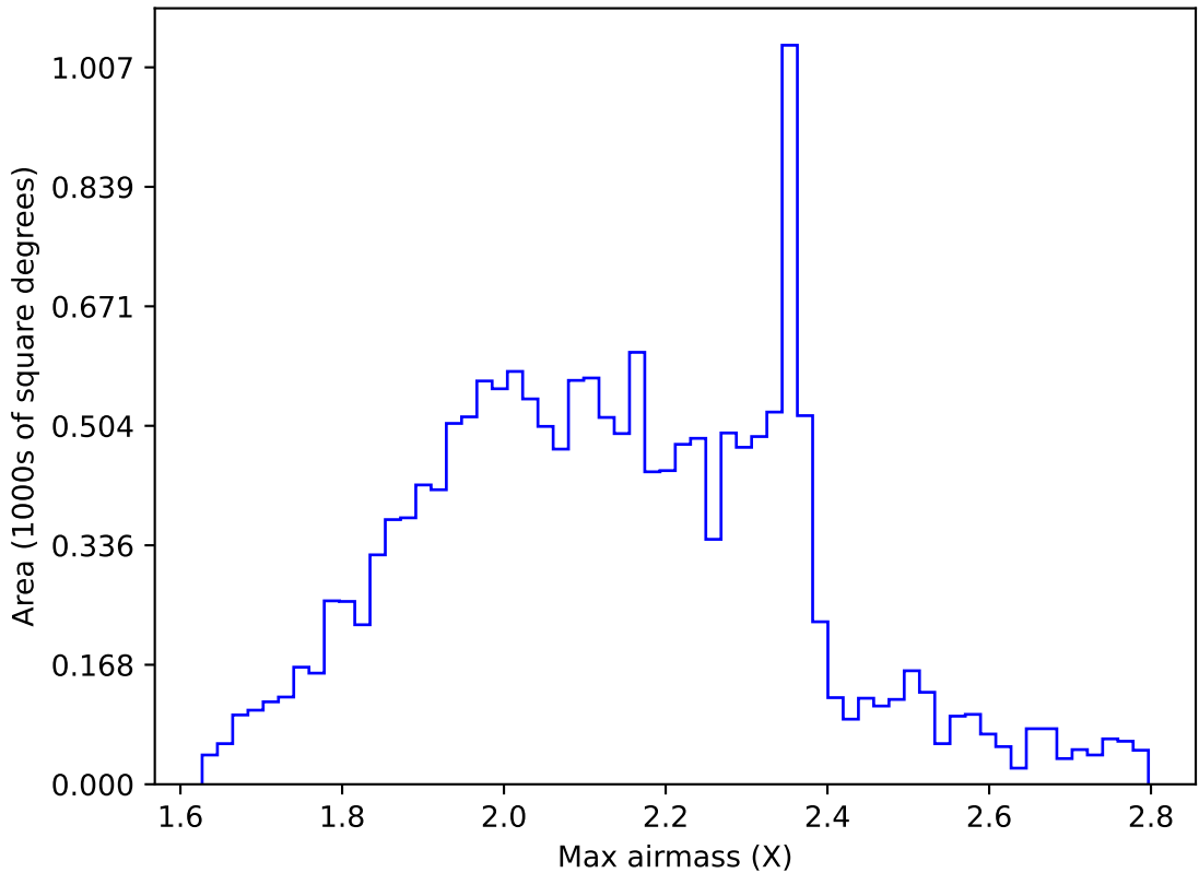
too_elab_heavy_r128_d3_gz_v3.4_10yrs WFD g band: Max airmass
