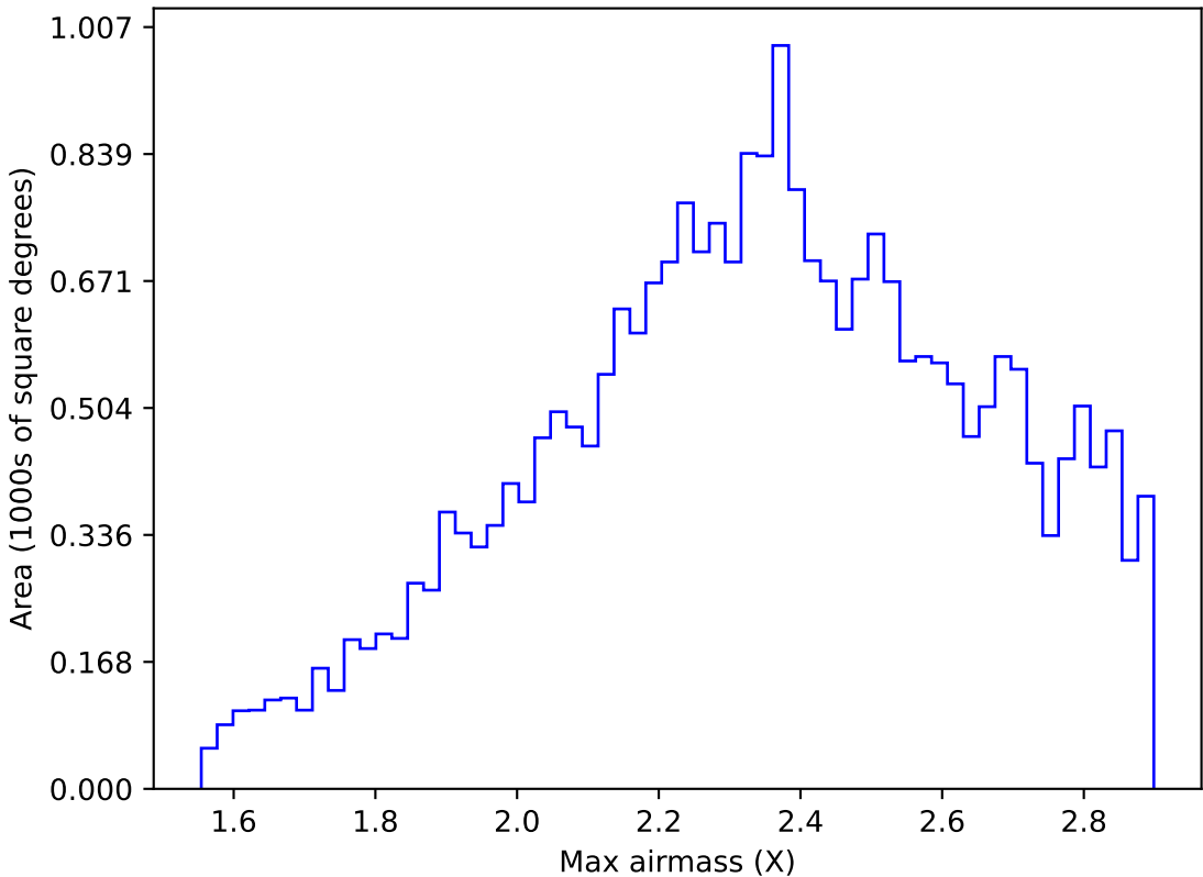
too_elab_heavy_r128_d3_gz_v3.4_10yrs All sky z band: Max airmass
