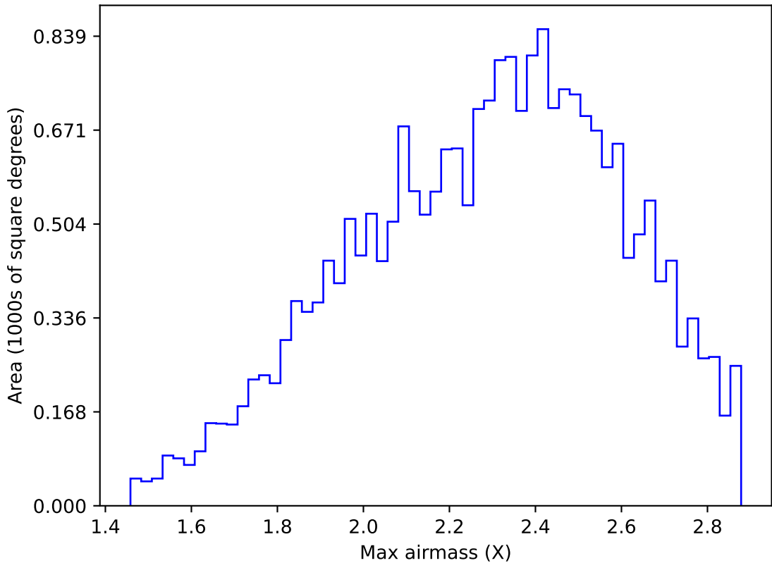
too_elab_heavy_r128_d3_gz_v3.4_10yrs All sky y band: Max airmass
