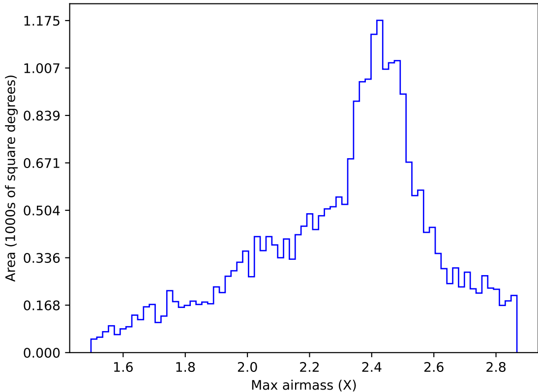
too_elab_heavy_r128_d3_gz_v3.4_10yrs All sky r band: Max airmass
