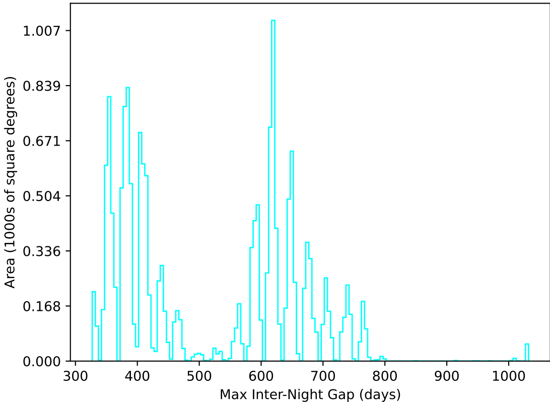
too_elab_heavy_r128_d3_gz_v3.4_10yrs WFD u band: Max Inter-Night Gap
