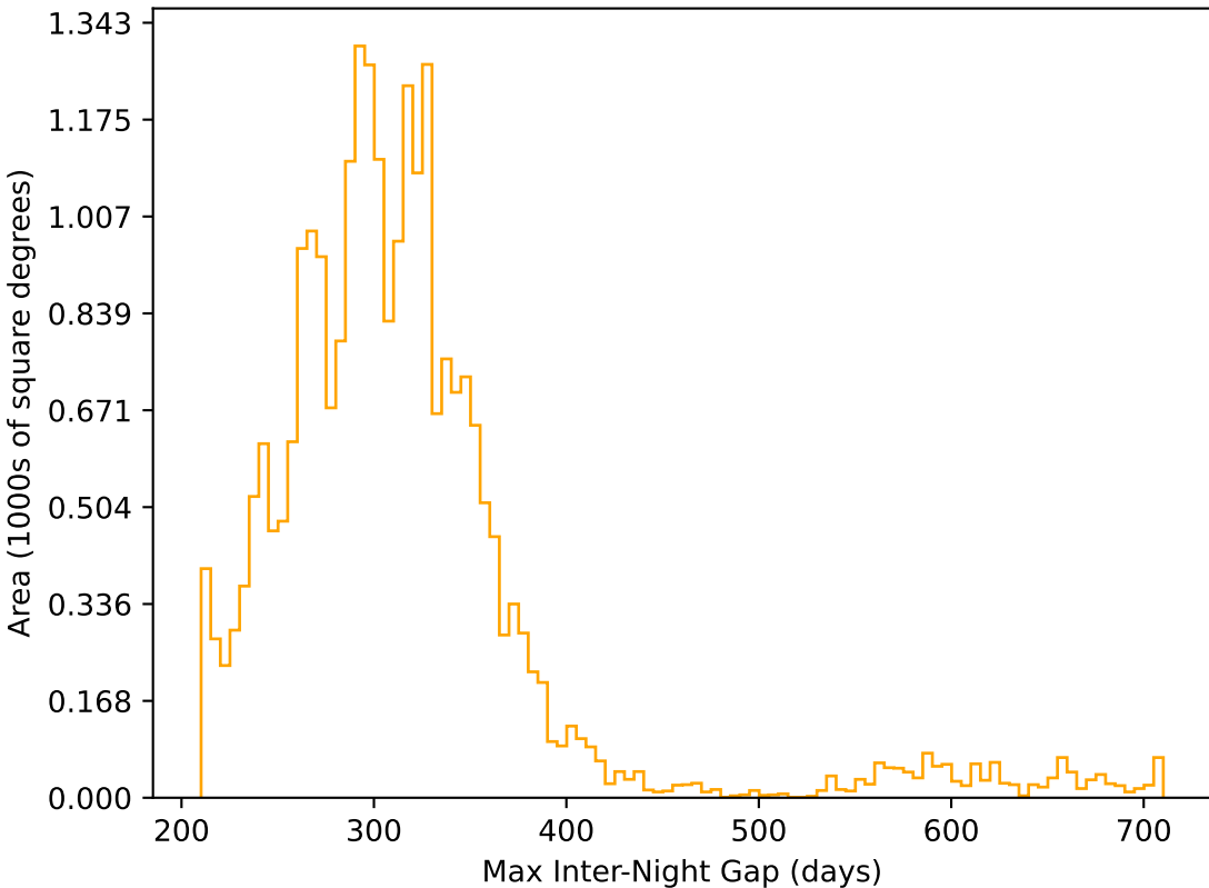
too_elab_heavy_r128_d3_gz_v3.4_10yrs All sky r band: Max Inter-Night Gap
