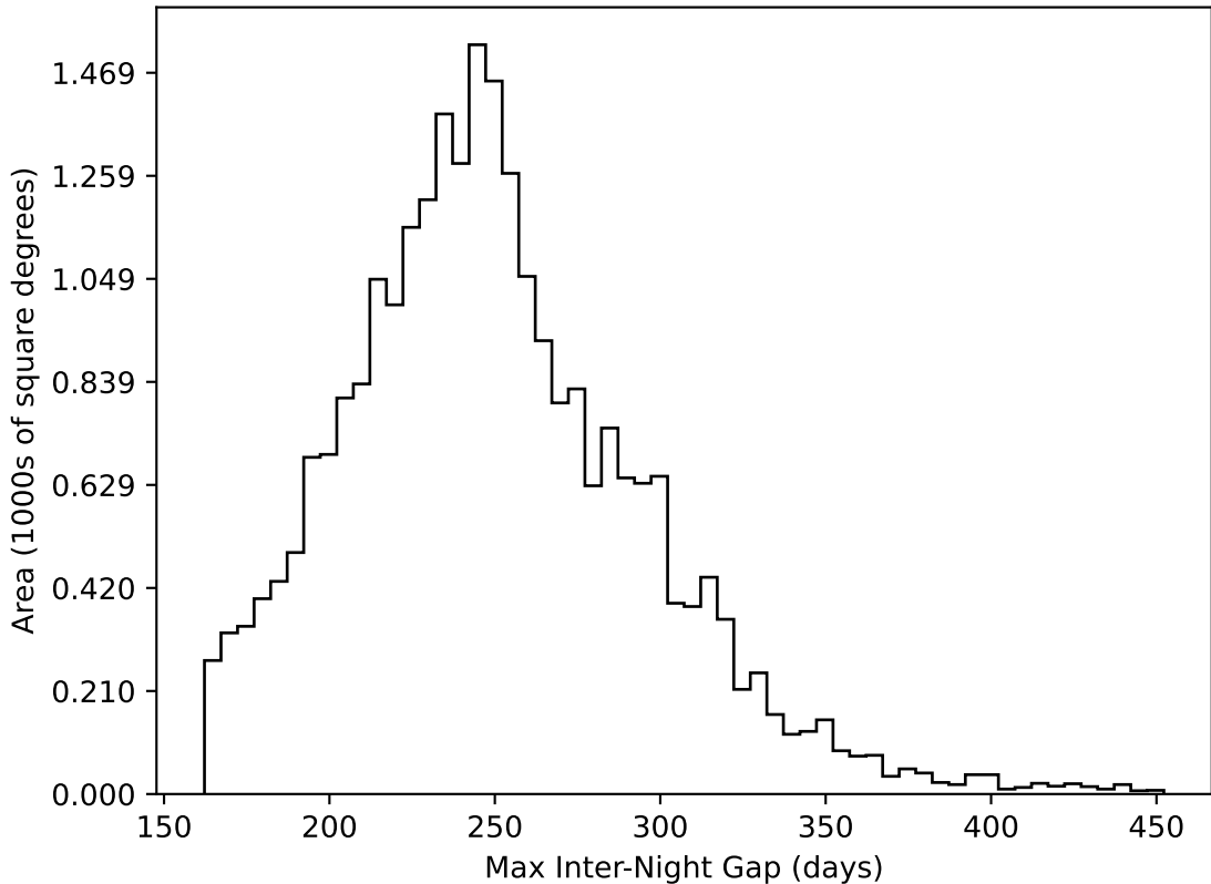
too_elab_heavy_r128_d3_gz_v3.4_10yrs All sky all bands: Max Inter-Night Gap
