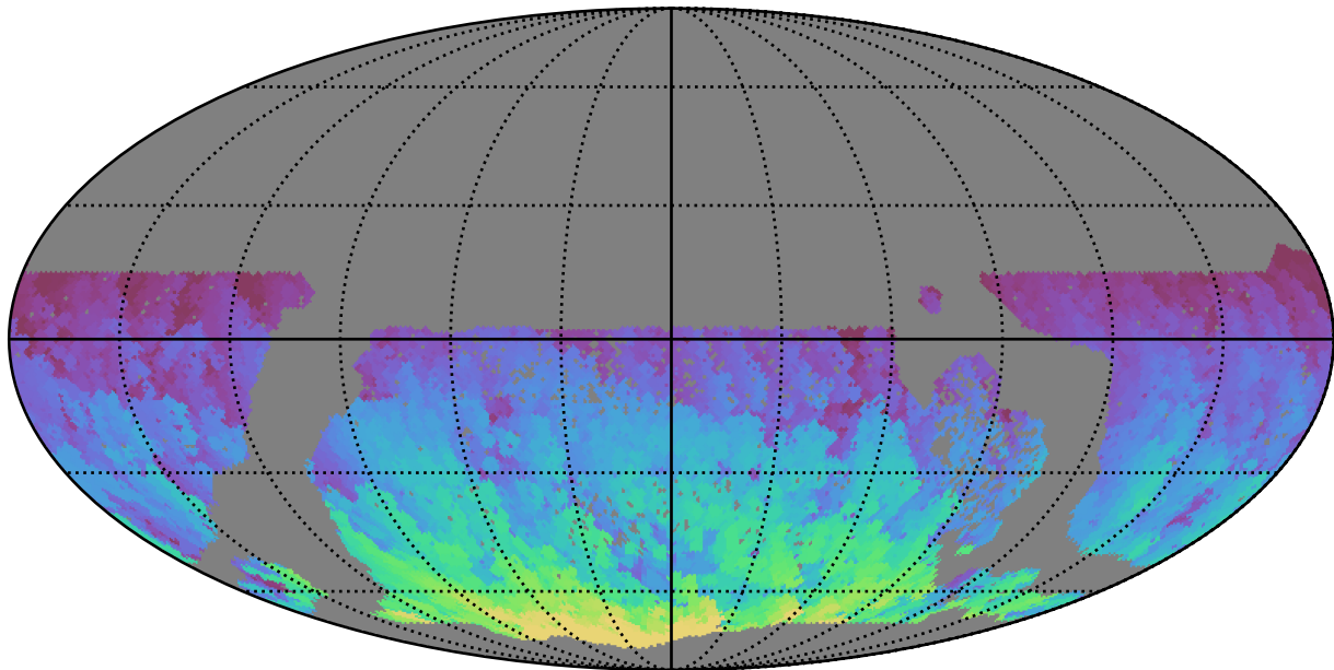
too_elab_heavy_r128_d3_gz_v3.4_10yrs WFD z band: Max HA
