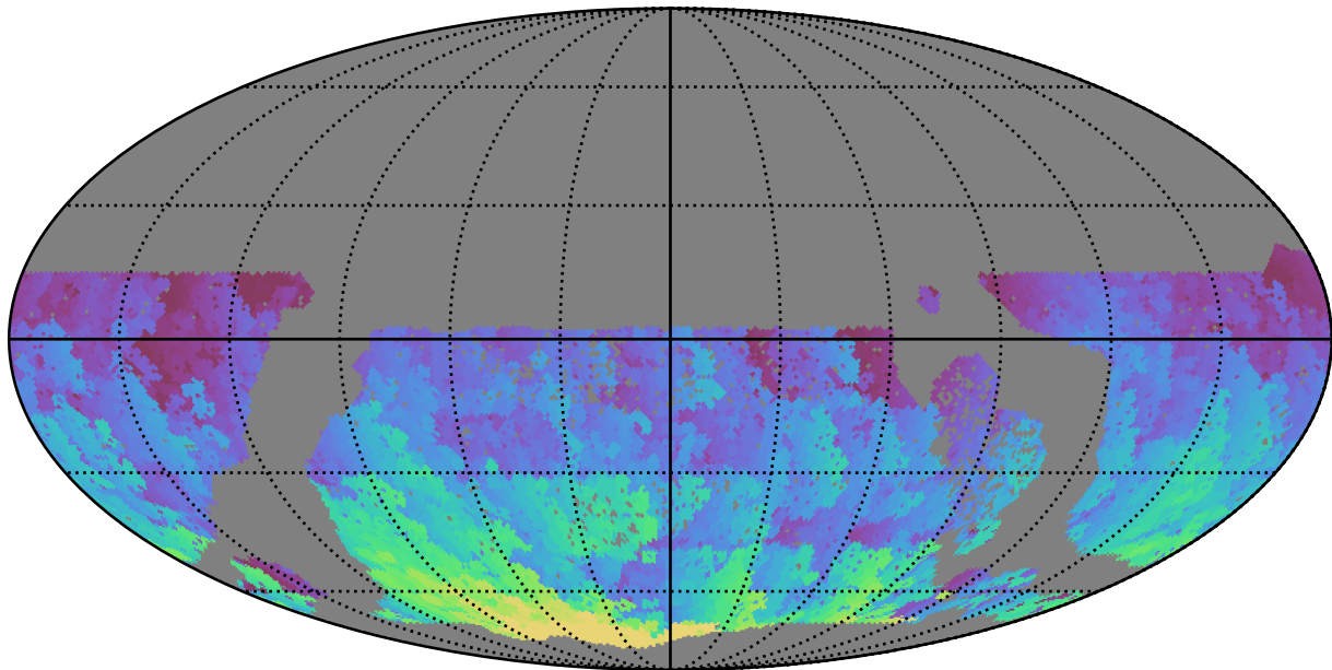
too_elab_heavy_r128_d3_gz_v3.4_10yrs WFD u band: Max HA
