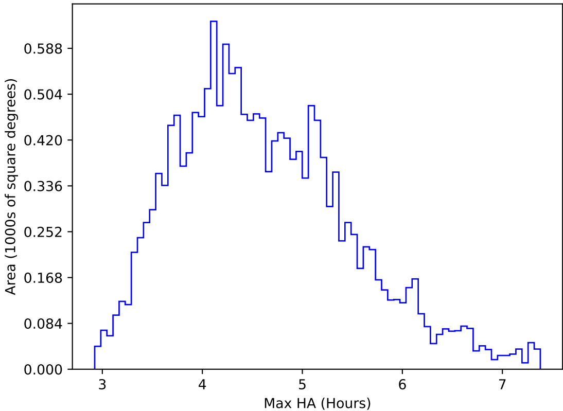
too_elab_heavy_r128_d3_gz_v3.4_10yrs WFD r band: Max HA
