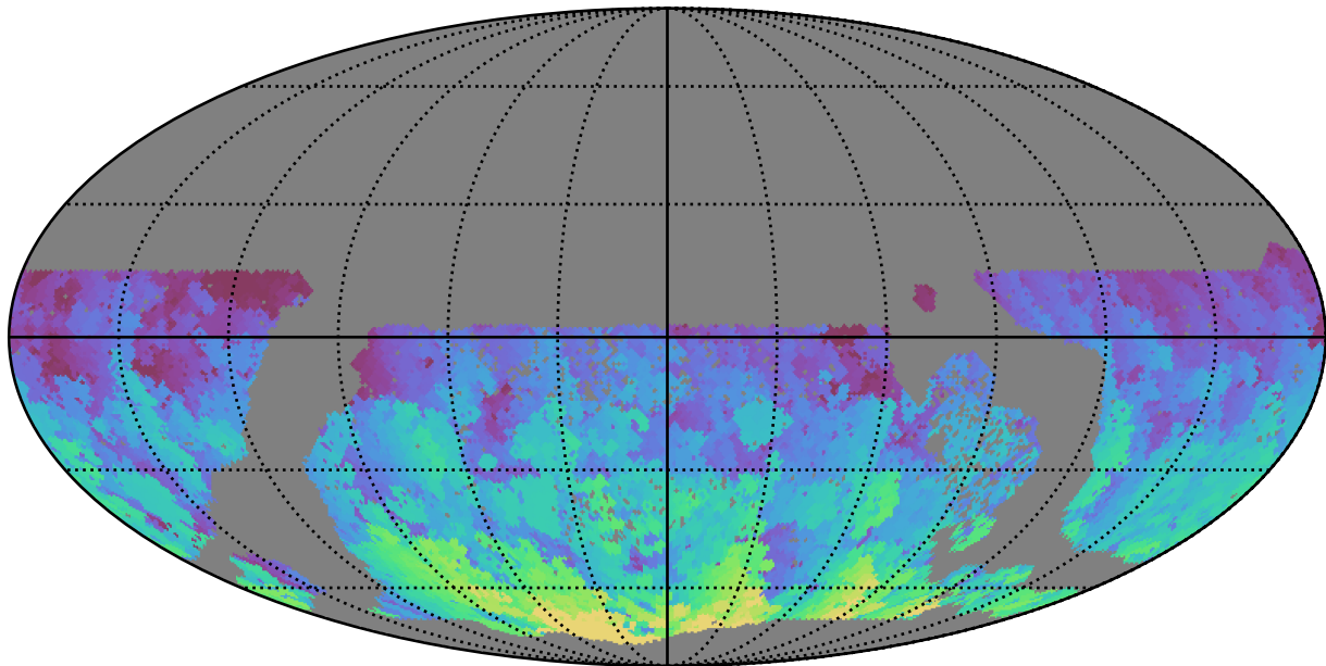
too_elab_heavy_r128_d3_gz_v3.4_10yrs WFD g band: Max HA
