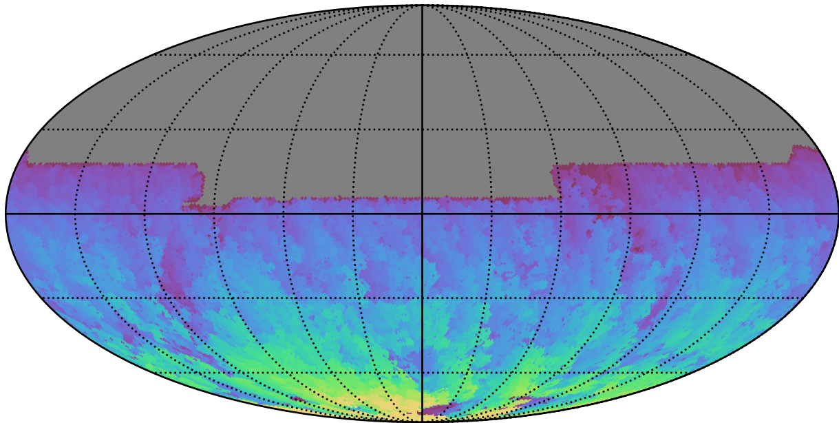
too_elab_heavy_r128_d3_gz_v3.4_10yrs All sky y band: Max HA
