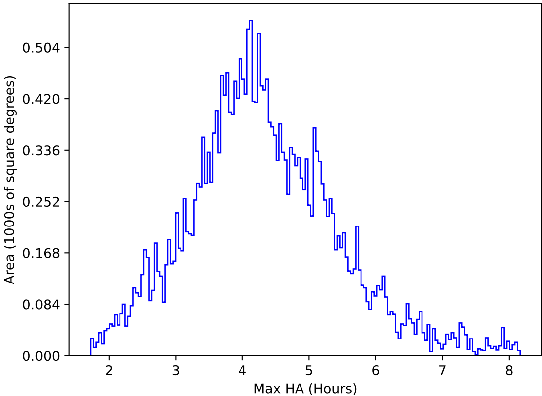
too_elab_heavy_r128_d3_gz_v3.4_10yrs All sky r band: Max HA
