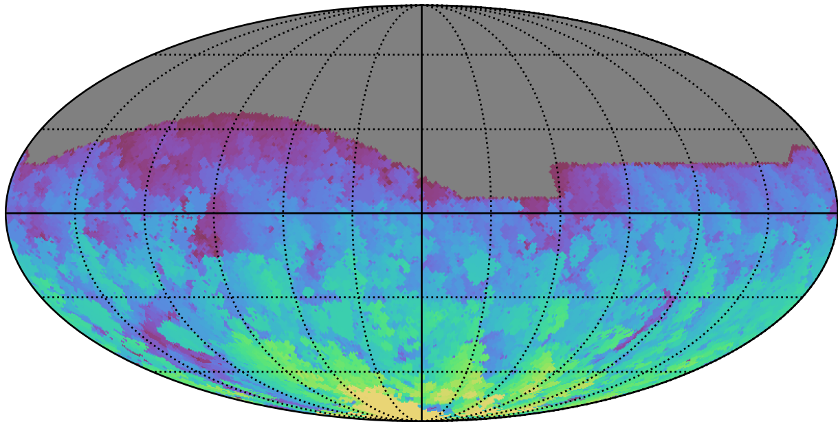
too_elab_heavy_r128_d3_gz_v3.4_10yrs All sky g band: Max HA
