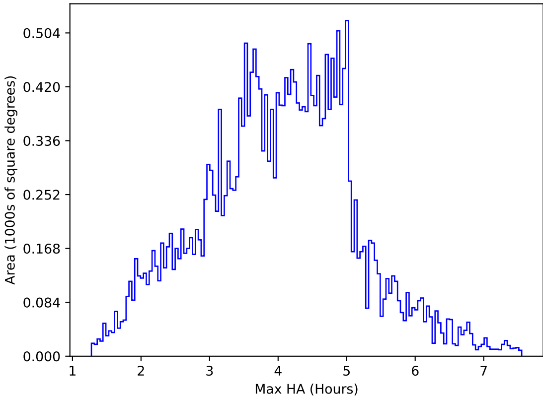
too_elab_heavy_r128_d3_gz_v3.4_10yrs All sky g band: Max HA
