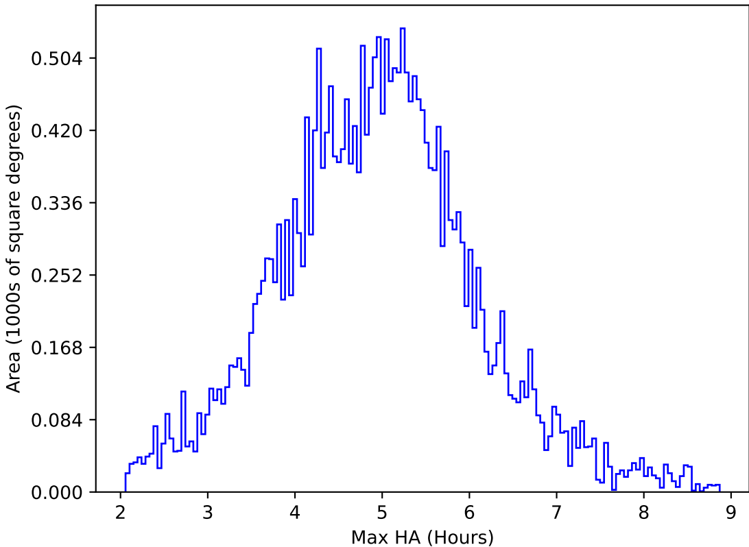
too_elab_heavy_r128_d3_gz_v3.4_10yrs All sky all bands: Max HA
