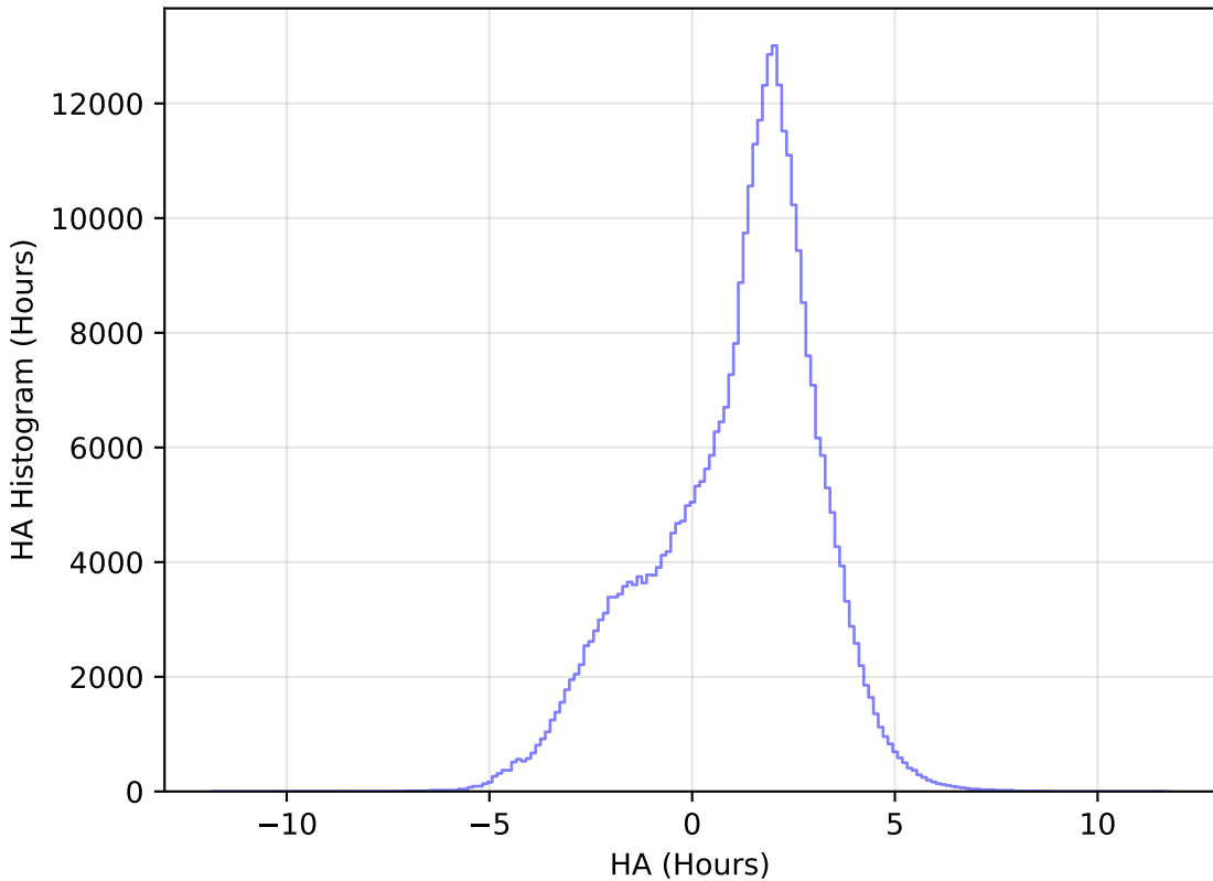
too_elab_heavy_r128_d3_gz_v3.4_10yrs WFD y band: HA Histogram
