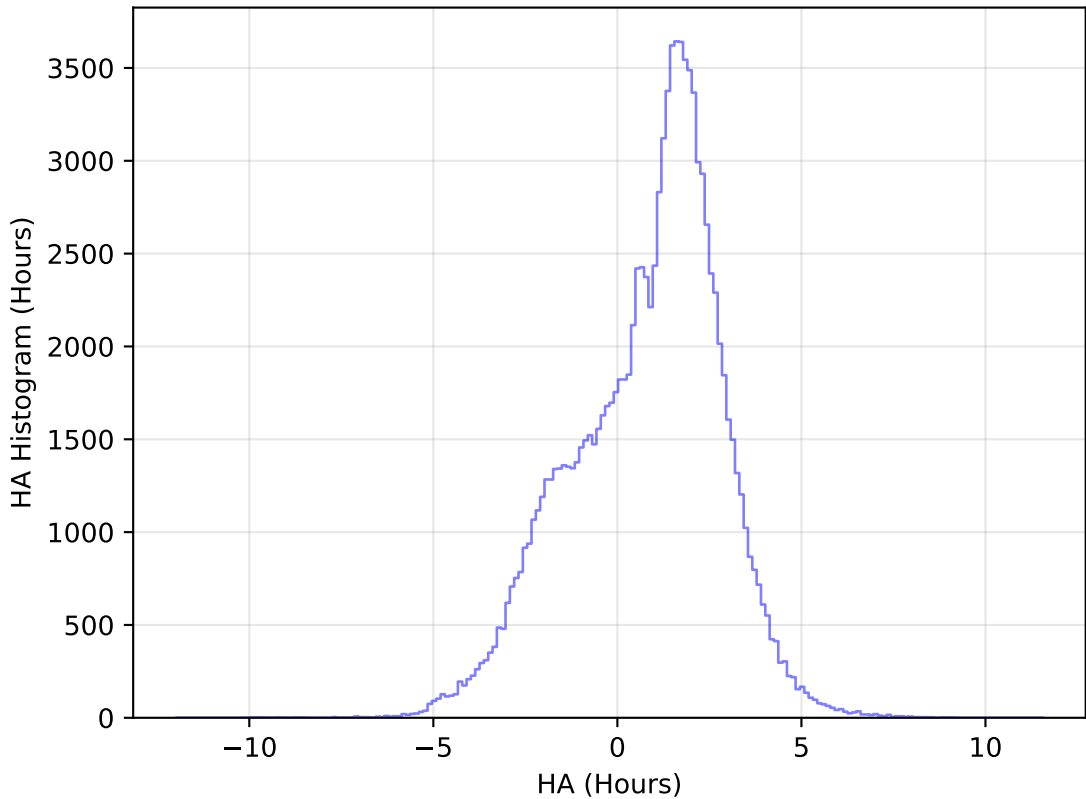
too_elab_heavy_r128_d3_gz_v3.4_10yrs WFD u band: HA Histogram
