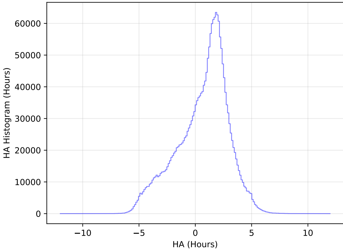
too_elab_heavy_r128_d3_gz_v3.4_10yrs WFD all bands: HA Histogram
