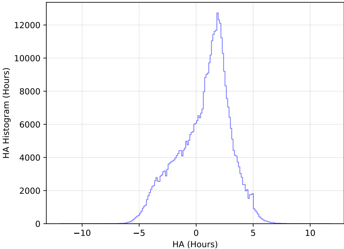
too_elab_heavy_r128_d3_gz_v3.4_10yrs All sky z band: HA Histogram
