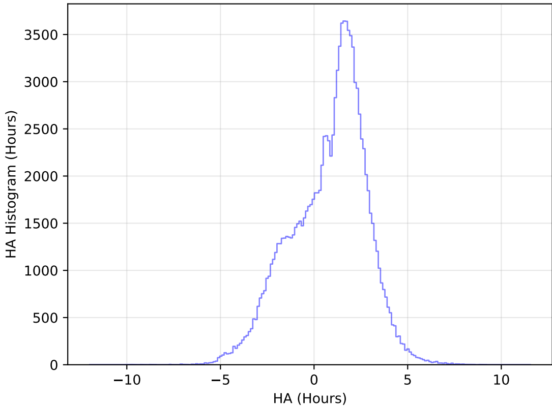
too_elab_heavy_r128_d3_gz_v3.4_10yrs All sky u band: HA Histogram
