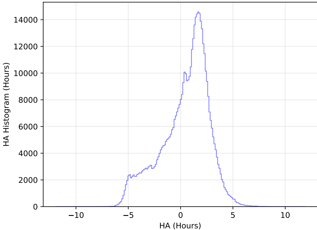
too_elab_heavy_r128_d3_gz_v3.4_10yrs All sky r band: HA Histogram
