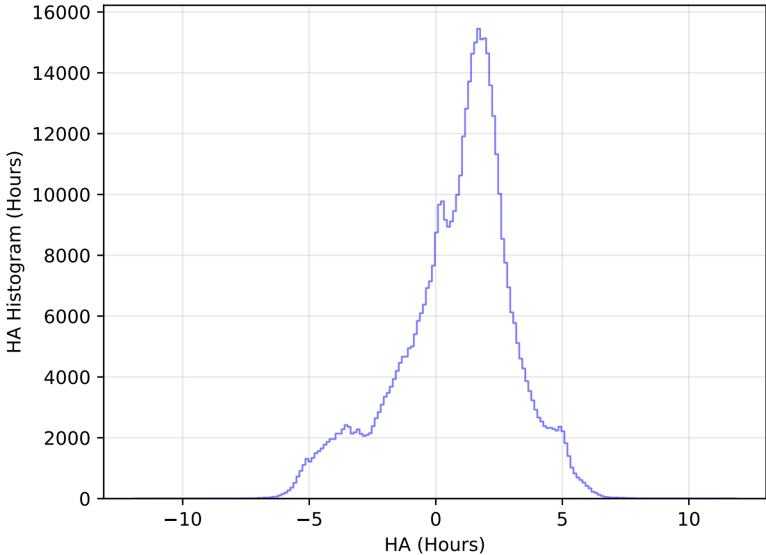
too_elab_heavy_r128_d3_gz_v3.4_10yrs All sky i band: HA Histogram
