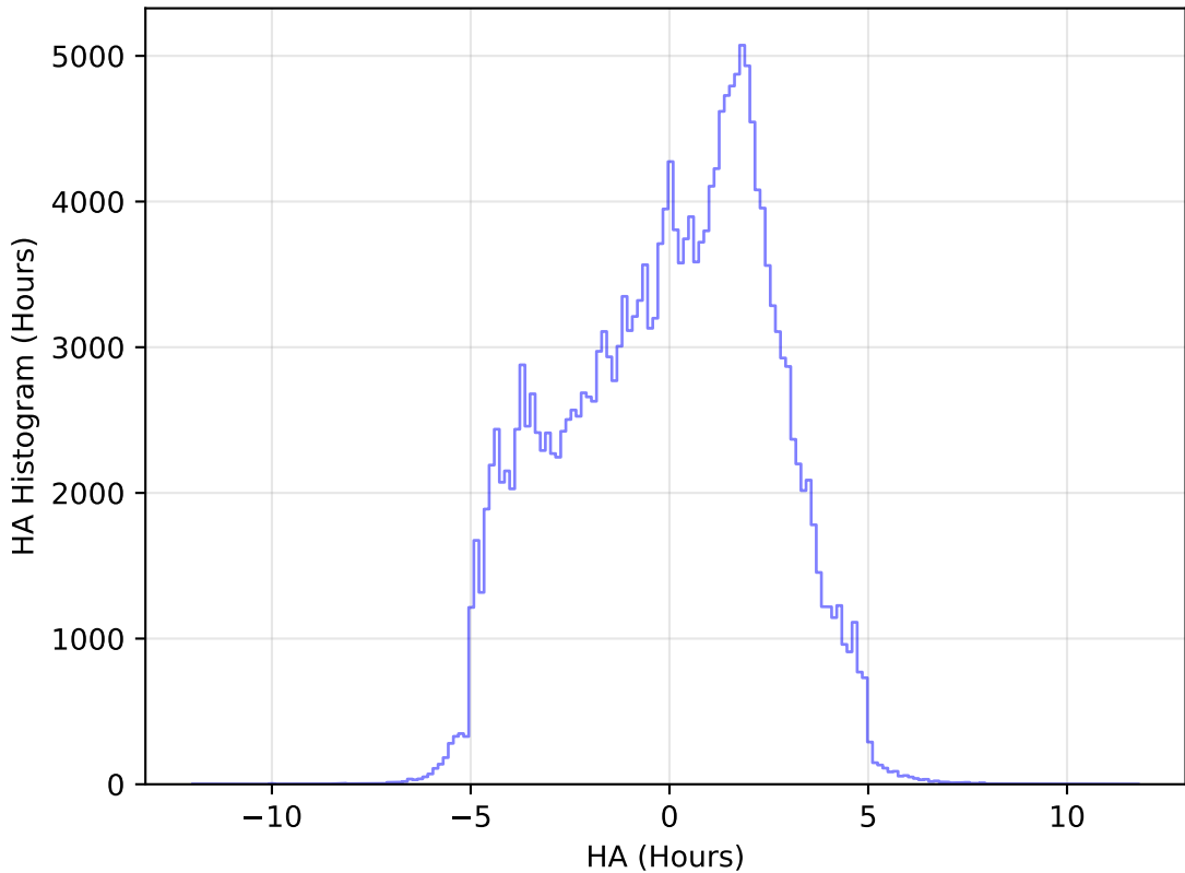
too_elab_heavy_r128_d3_gz_v3.4_10yrs All sky g band: HA Histogram
