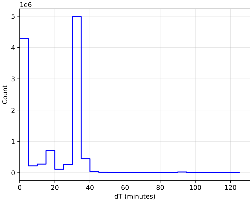
too_elab_heavy_r128_d3_gz_v3.4_10yrs WFD: DeltaT Histogram
