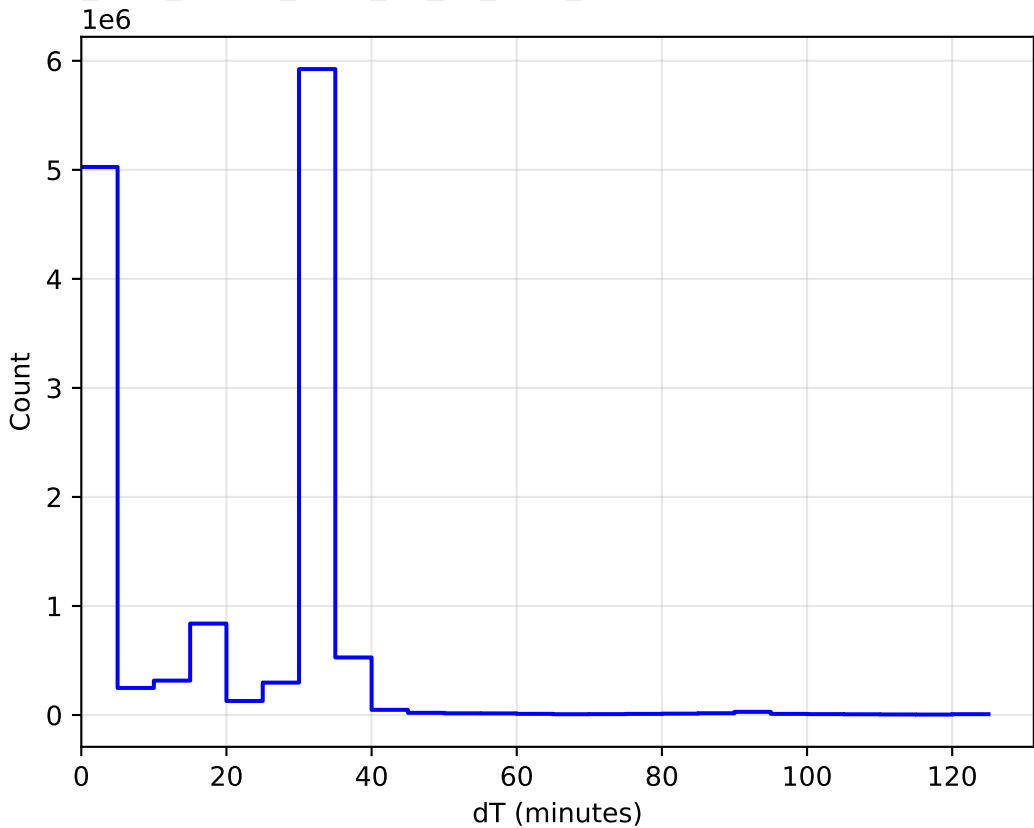
too_elab_heavy_r128_d3_gz_v3.4_10yrs All sky: DeltaT Histogram
