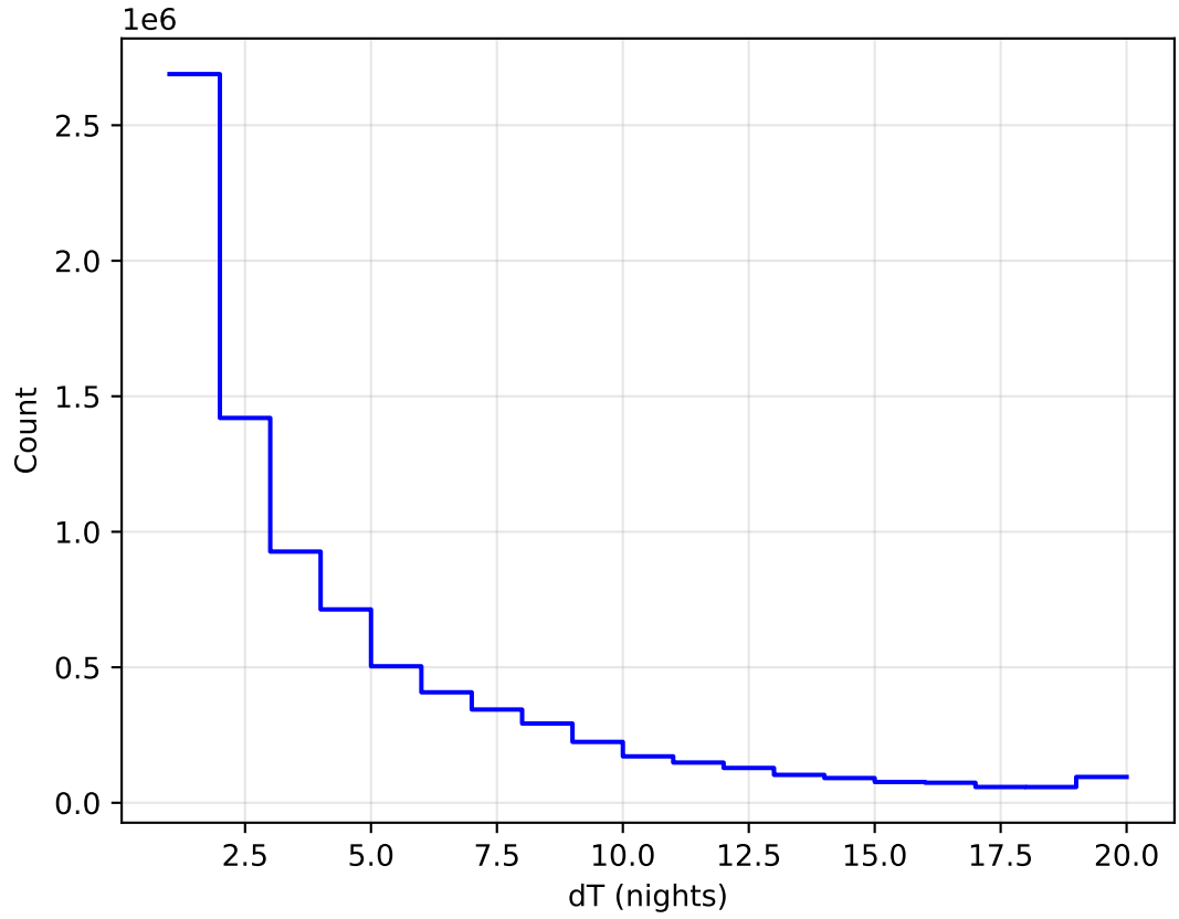
too_elab_heavy_r128_d3_gz_v3.4_10yrs All sky all bands: DeltaNight Histogram
