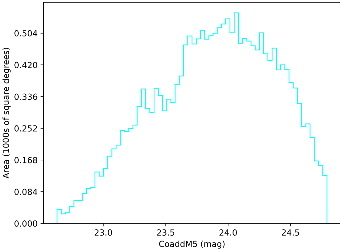
too_elab_heavy_r128_d3_gz_v3.4_10yrs Yr 3-4 u band: CoaddM5
