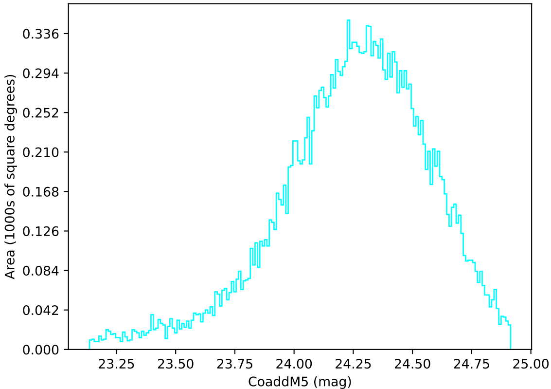
too_elab_heavy_r128_d3_gz_v3.4_10yrs Yr 1 u band: CoaddM5
