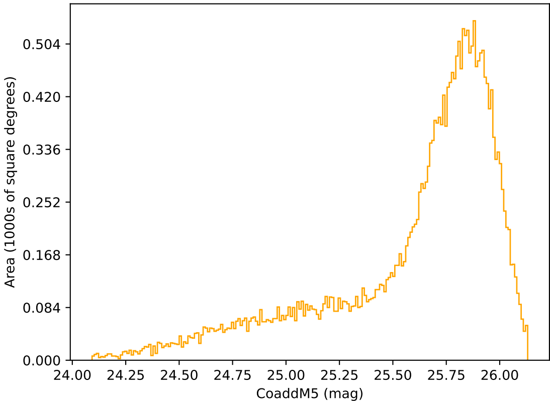
too_elab_heavy_r128_d3_gz_v3.4_10yrs Yr 1 r band: CoaddM5
