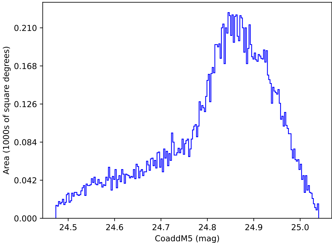
too_elab_heavy_r128_d3_gz_v3.4_10yrs WFD y band: CoaddM5
