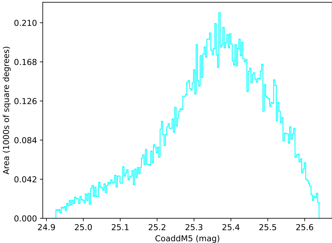
too_elab_heavy_r128_d3_gz_v3.4_10yrs WFD u band: CoaddM5
