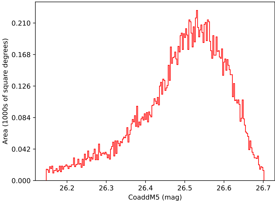
too_elab_heavy_r128_d3_gz_v3.4_10yrs WFD i band: CoaddM5
