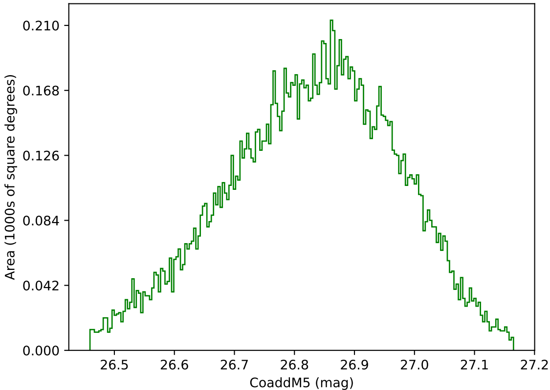
too_elab_heavy_r128_d3_gz_v3.4_10yrs WFD g band: CoaddM5
