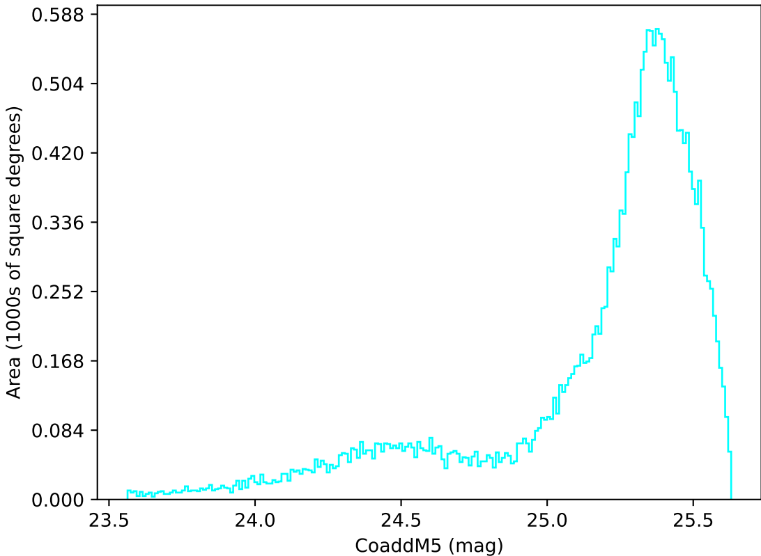
too_elab_heavy_r128_d3_gz_v3.4_10yrs All sky u band: CoaddM5
