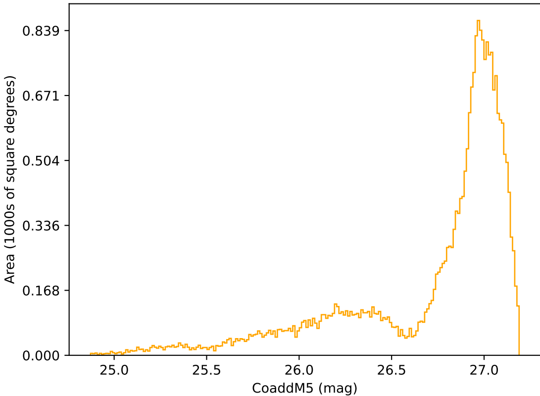
too_elab_heavy_r128_d3_gz_v3.4_10yrs All sky r band: CoaddM5
