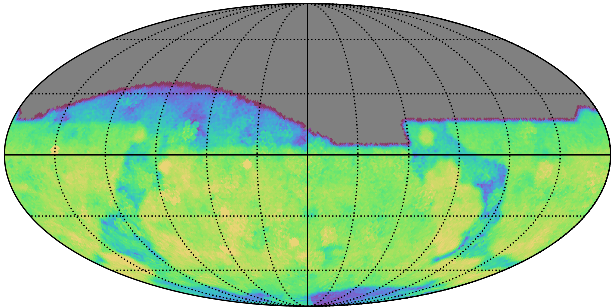
too_elab_heavy_r128_d3_gz_v3.4_10yrs All sky g band: CoaddM5
