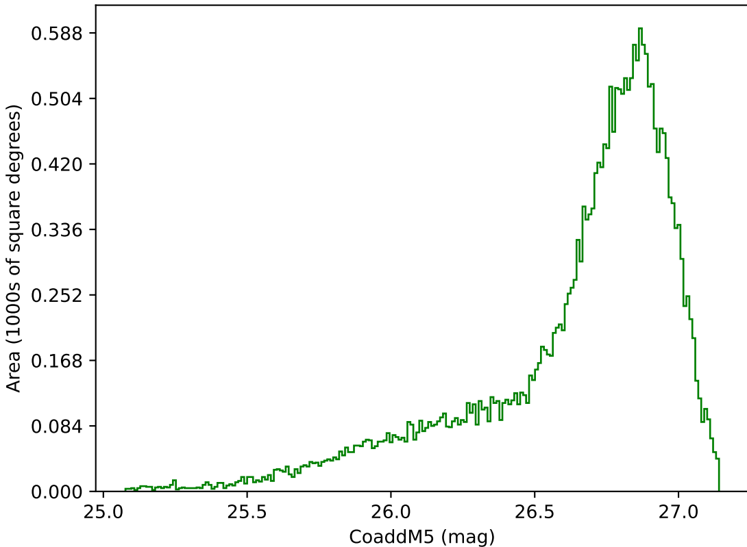
too_elab_heavy_r128_d3_gz_v3.4_10yrs All sky g band: CoaddM5
