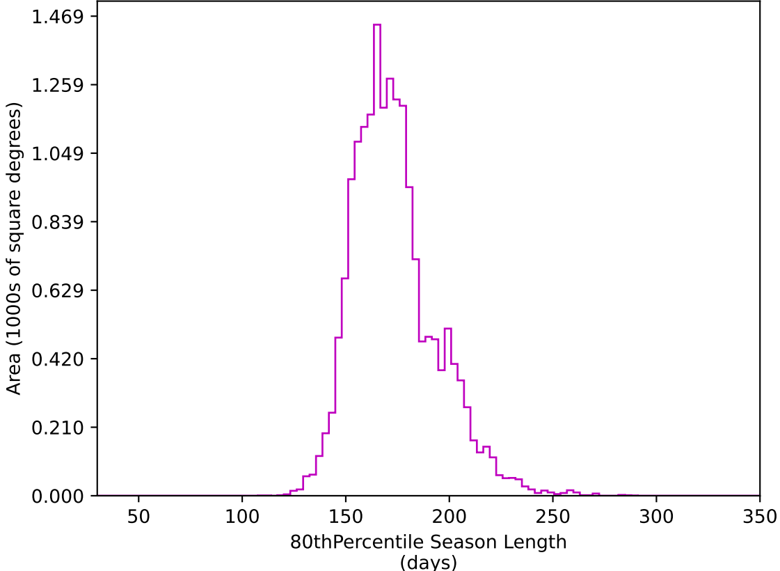
too_elab_heavy_r128_d3_gz_v3.4_10yrs WFD z band: 80thPercentile Season Length
