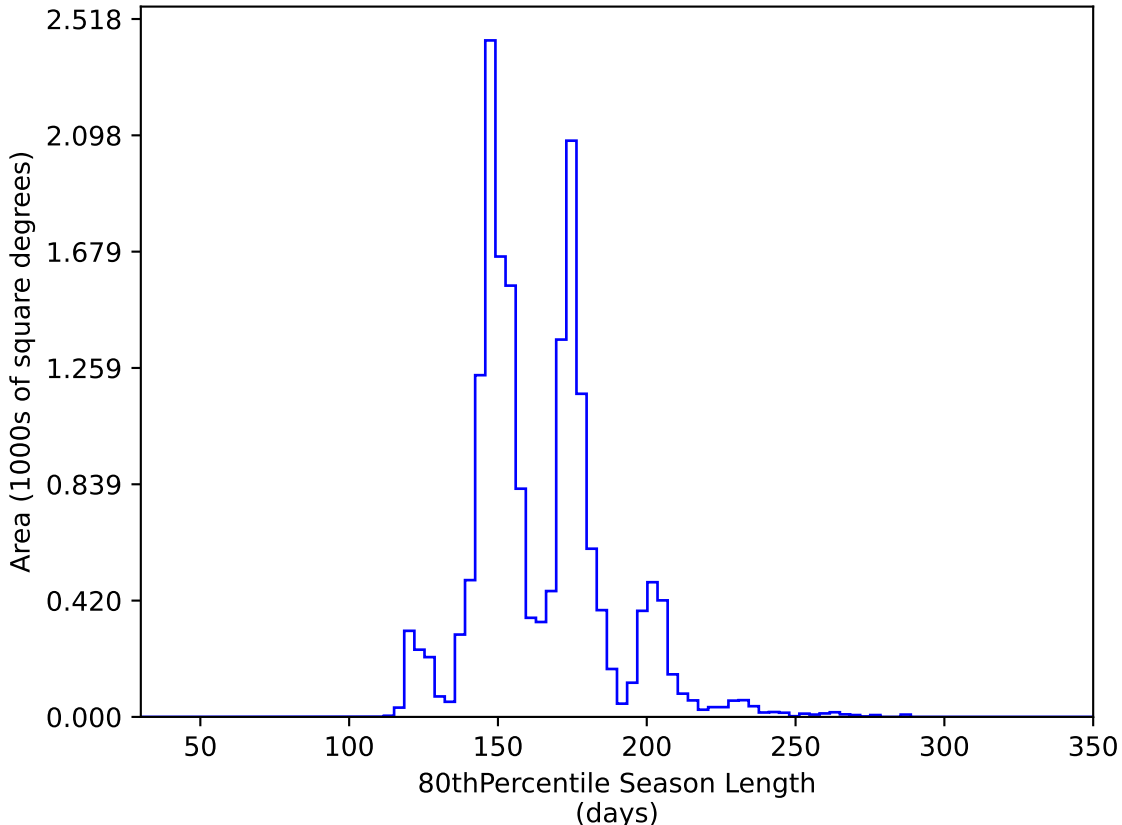
too_elab_heavy_r128_d3_gz_v3.4_10yrs WFD y band: 80thPercentile Season Length
