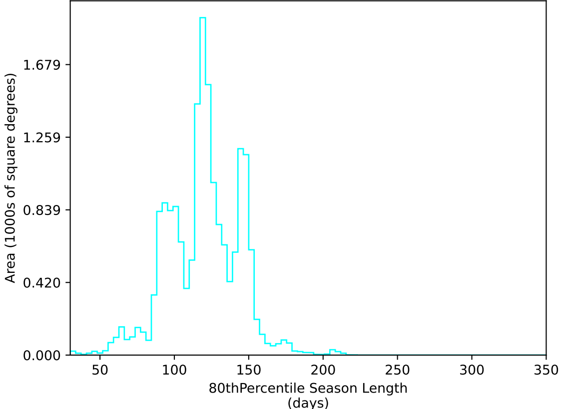
too_elab_heavy_r128_d3_gz_v3.4_10yrs WFD u band: 80thPercentile Season Length
