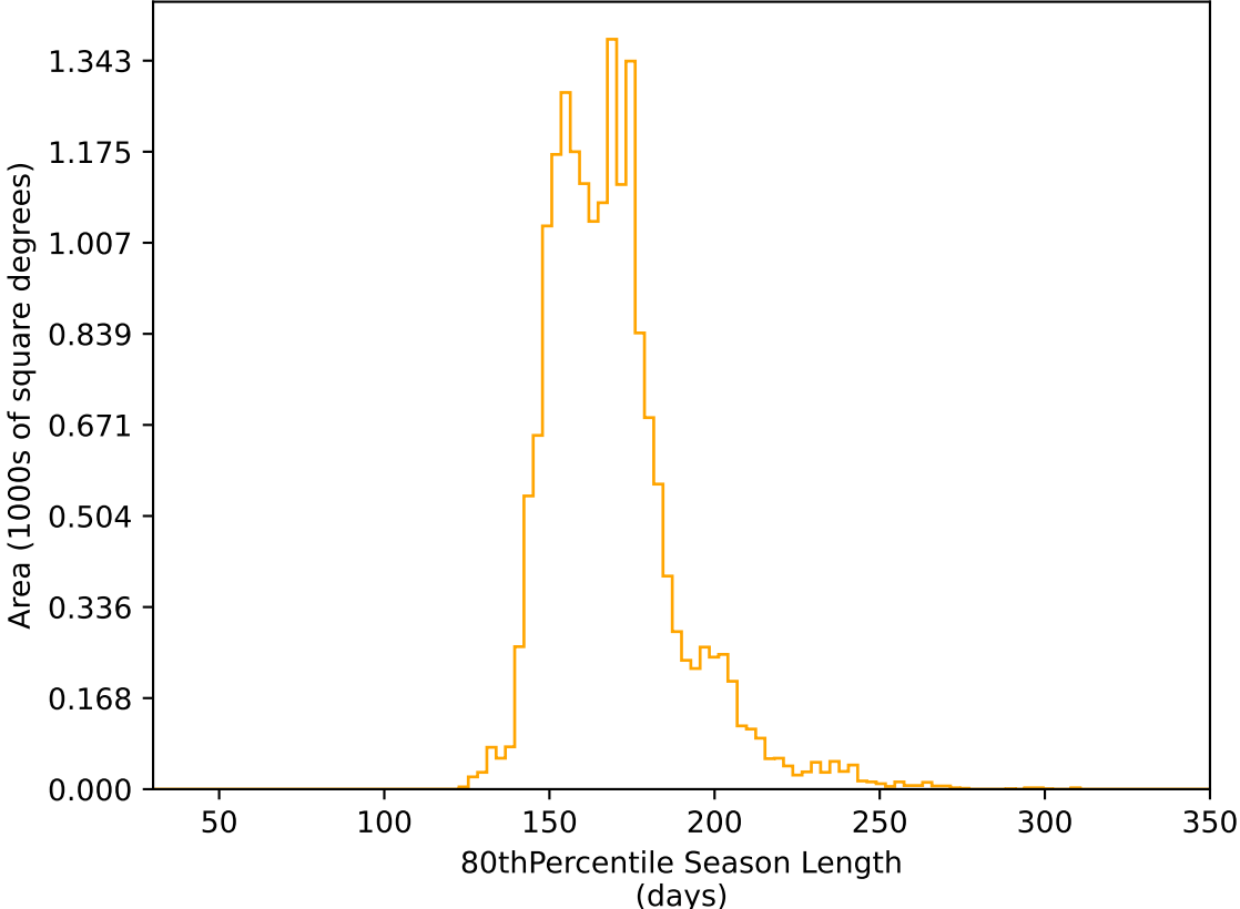
too_elab_heavy_r128_d3_gz_v3.4_10yrs WFD r band: 80thPercentile Season Length
