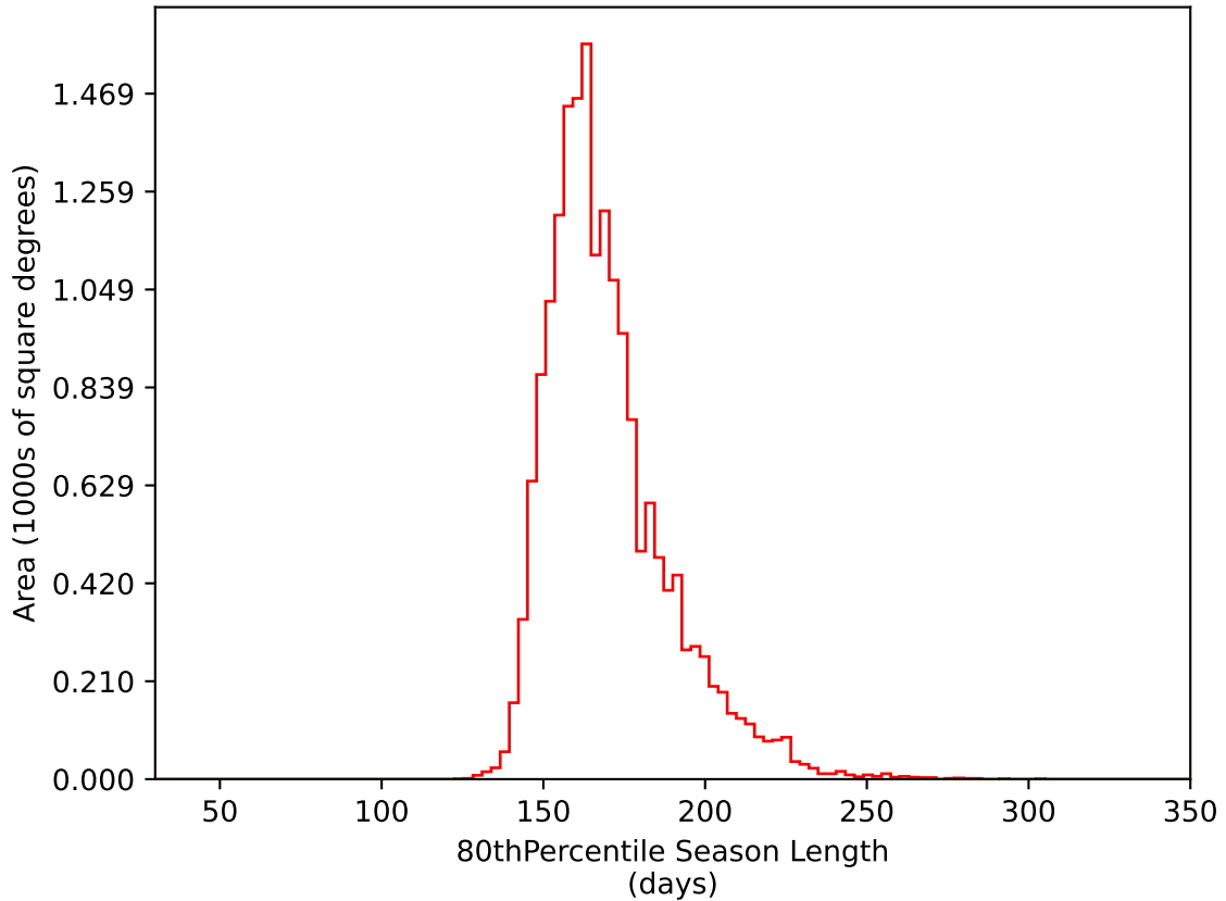
too_elab_heavy_r128_d3_gz_v3.4_10yrs WFD i band: 80thPercentile Season Length
